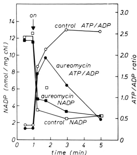
Fig. 8. Light-dependent changes in the ratios of ATP to ADP and in NADP levels in intact chloroplasts as a function of illumination time with and without 45 \mu M aureomycin present. The chloroplast suspension contained 1 mM 3-phosphoglycerate. The intensity of red light was 400 \text{Wm}^{-2} .
